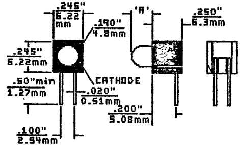
Model PC190/200
